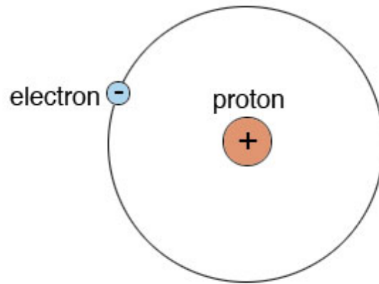
Hydrogen Atom
