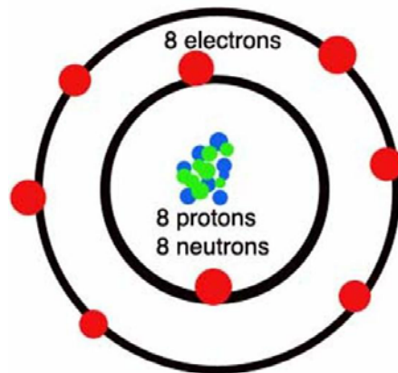
Oxygen Atom
